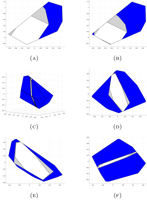
FIGURE 2. (a) Sets of Example 1 with u \in [-2, 2] . (b) Sets of Example 1 with u \in [-1, 1] . (c) Sets of Example 2. (d) 2D slice of (c) in z-axis. (e) 2D slice of (c) in x-axis (e) 2D slice of (c) in y-axis Legend: Original set D (blue); Exact MCIS of D (light gray); Controlled invariant set \mathcal{D} from Algorithm 1 (white).
