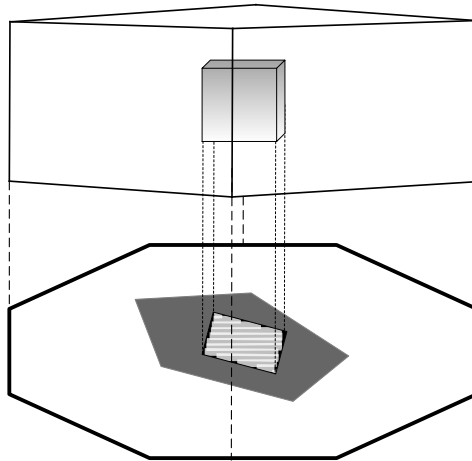
FIGURE 1. Illustration of domain lifting. Octagon is the original set D_c . Transparent hyper-rectangle is an instantiation of the hyper-rectangles whose union represents the lifted set D_c^\ell . Gradient cube is the MCIS in the higher dimension. Light grey rectangle is the controlled invariant set obtained after projection. Dark grey polygon is the exact MCIS.
